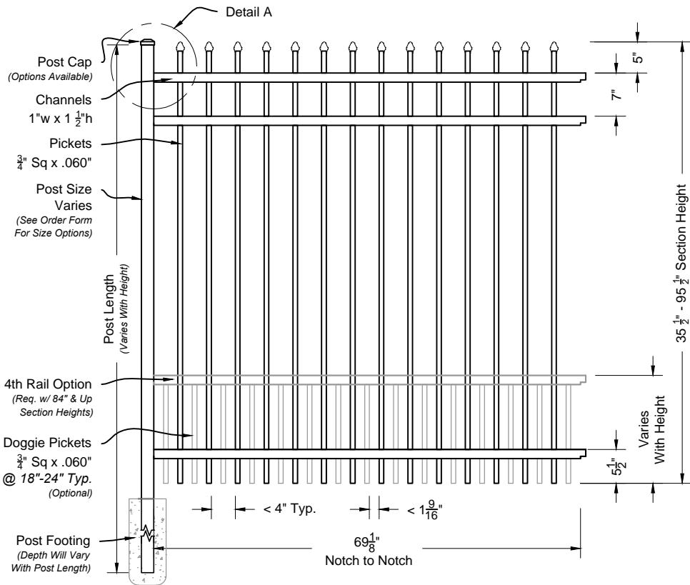
i 01 Maine #203 6ft Fence Panel Shown As Commerical Series Scale: NTS
