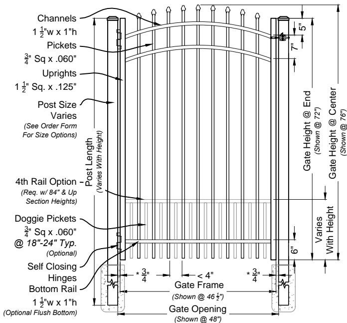
i 02 Maine Single Walk Gate #3033 Arched Rail Option Scale: NTS
