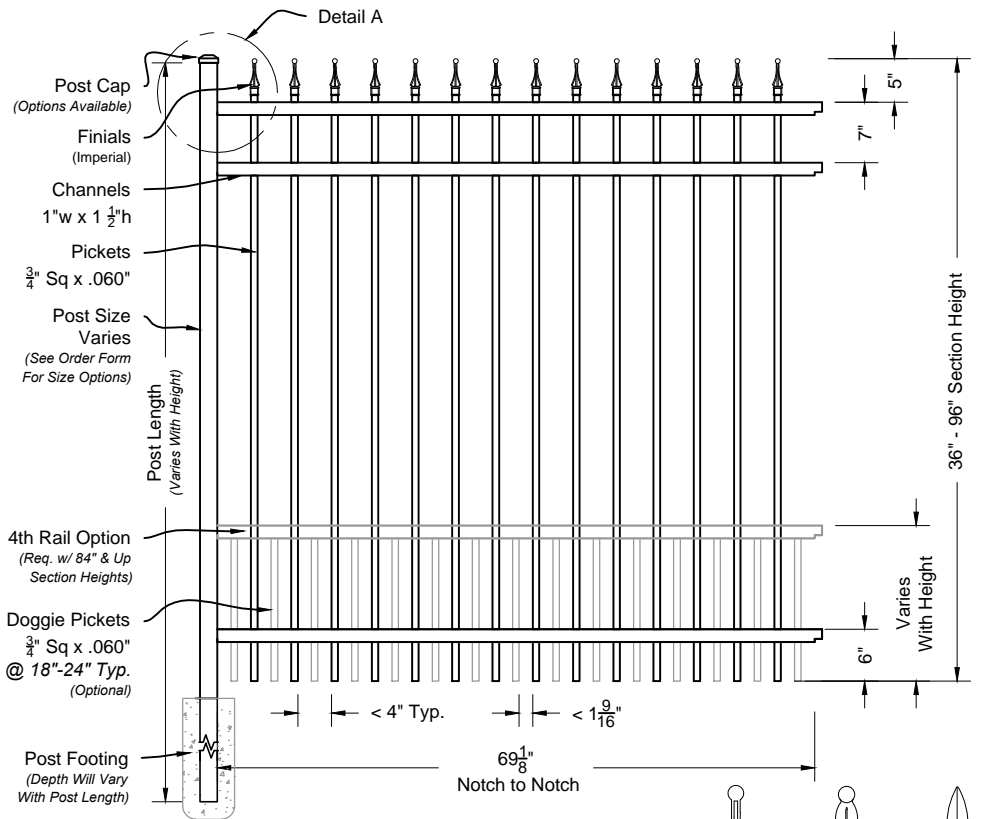
i 01 Finials #600 6ft Fence Panel Shown As Commercial Series Scale: NTS
