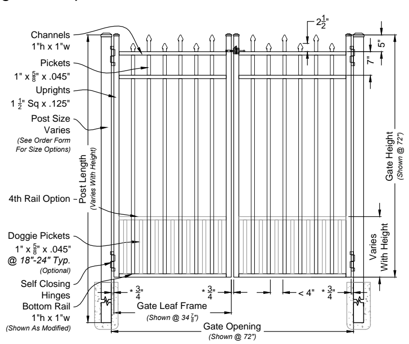
i 03 Californian Double Walk Gate #6200M Straight Rail Option Scale: NTS
