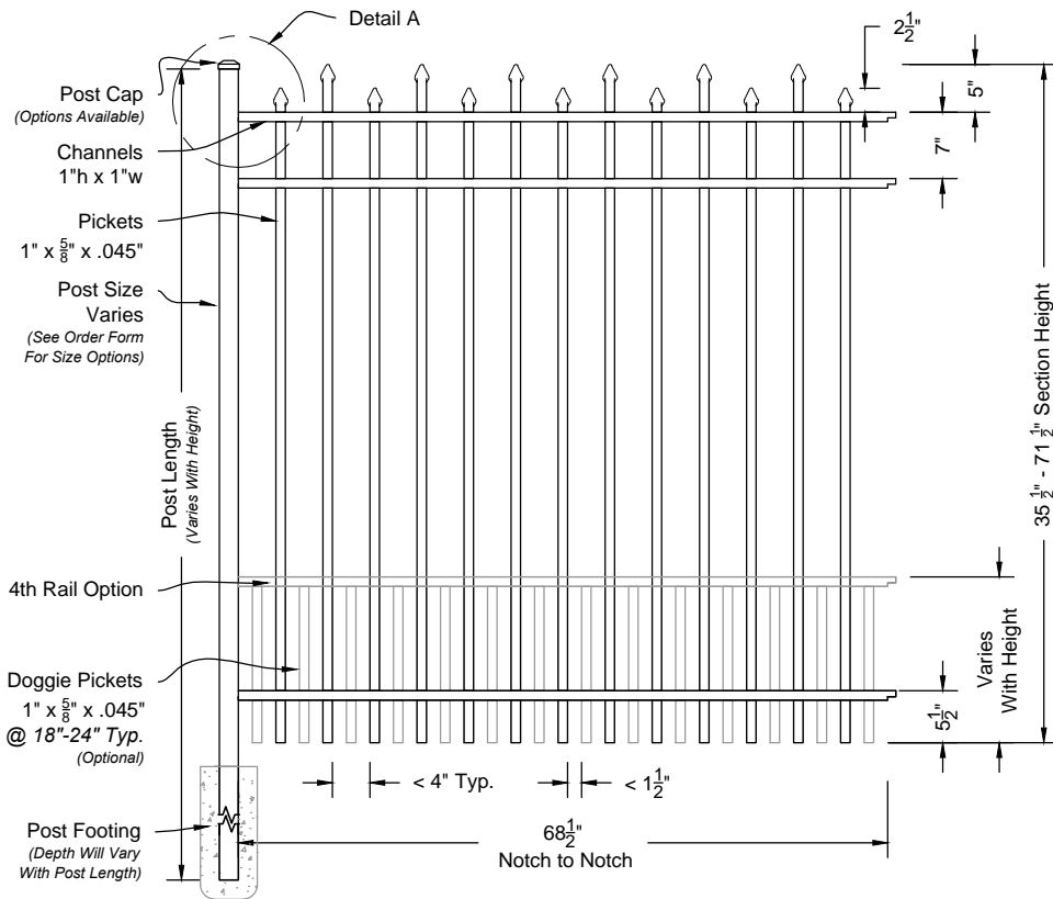
i 01 Californian #200 6ft Fence Panel Shown As Parkway Series Scale: NTS
